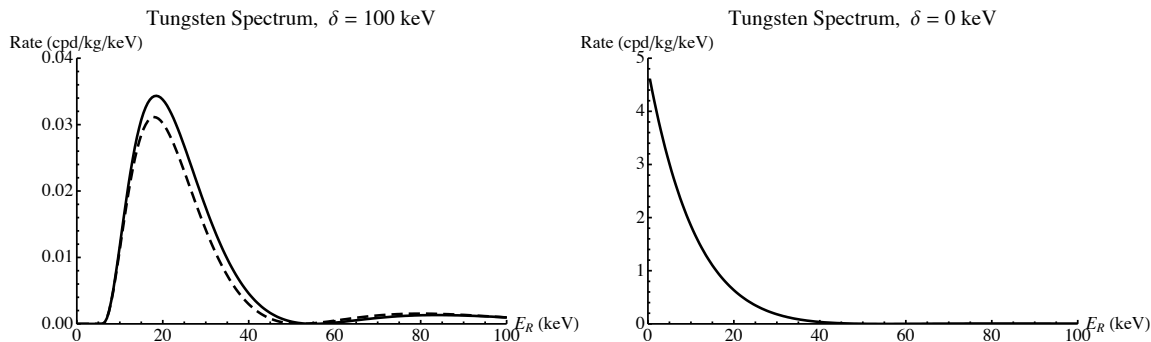
Figure 1. Recoil energy spectrum for scattering off of tungsten. On the left the inelastic scattering rates are shown for the two choices of form factor: the Fermi Two-Parameter (dashed) and Helm (solid) form factor. Both choices show that iDM leads to a suppression of low-energy events. The right panel shows the recoil energy spectrum for elastic scattering; in this case the difference between the two form factors is negligible. For elastic scattering the recoil spectrum peaks at low E_R . All calculations assume M_\chi = 200 GeV, \sigma_n = 10^{-40} cm 2 and the SHM velocity distribution truncated at v_{\text{esc}} = 500 km/s.
