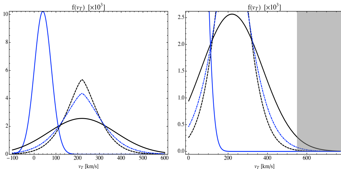
Figure 5. Left Panel: Tangential velocity distributions in the Earth rest frame. The solid black and blue lines show the SHM and Dark Disc distributions and the dashed and dot-dashed lines show the VL 220 and VL 270 distributions respectively. The Dark Disc distribution is peaked at 40 km/s. Right Panel: Detectable particle distributions in a germanium detector as a function of tangential velocity. The detectable region is shaded in grey. The left edge of the grey region corresponds to M_\chi = 500 GeV.
