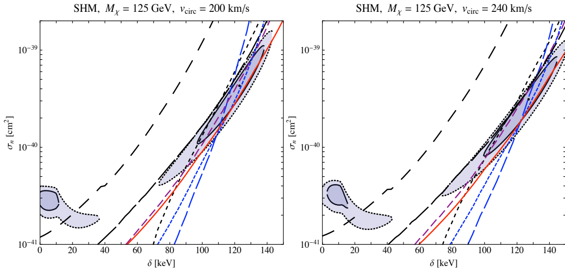
Figure 11. The exclusion limits for a local circular velocity of v_{\text{circ}} = 200 (left panel) and v_{\text{circ}} = 240 (right panel), for a WIMP mass of 125 GeV and using the SHM. One can see that the limits change a small amount and that the overall agreement with the DAMA results is slightly better for a lower circular velocity. However, the overall qualitative effect of changing the circular velocity is relatively small.
