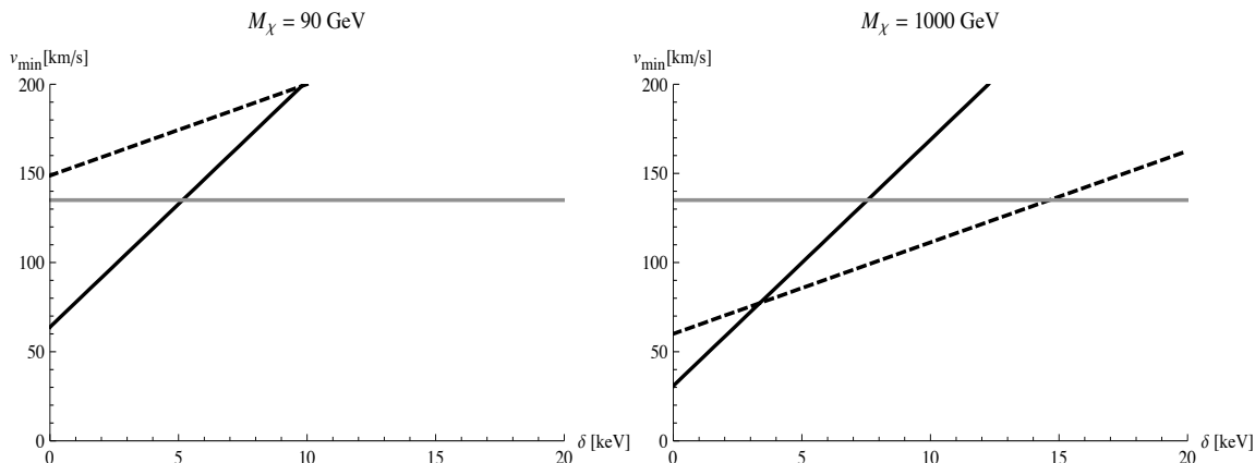
Figure 9. The minimum velocity for scattering at CRESST-II (Dashed) and DAMA (Solid). The velocities are calculated using eq. (2.1) and taking the experimental energy threshold. The DAMA line corresponds to channeled scattering and the gray line is roughly the maximum velocity at which the Dark Disk particles would be found. For \delta \geq 15 keV very few particles in the dark disc will scatter.
