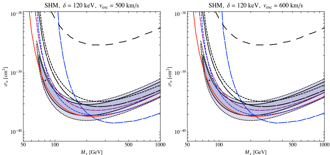
Figure 12. Exclusion limits for the SHM for v_{\text{esc}} = 500 km/s (left panel) and v_{\text{esc}} = 600 km/s (right panel). There is better agreement between experiments for lower escape velocity and the limits from CDMS II show the most sensitivity to the escape velocity.
